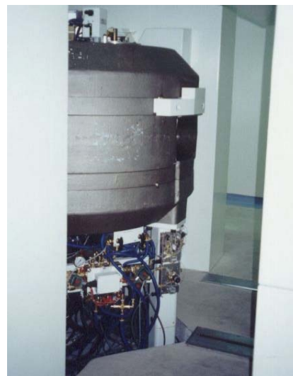
Figure 7: RDS-111 cyclotron installed at a hospital.
