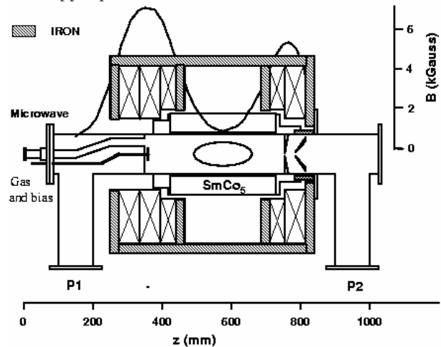
Figure 1: Schematic VEC-ECR
