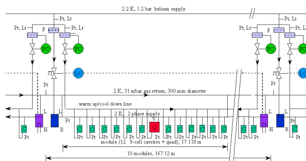
Fig. 2: Cryogenic string (C: cavity, Q: quadrupole, Pt: platinum sensor, Lt: low temperature sensor, F: flow meter, JT: Joule-Thomson valve, FC: flow control, LC: level control, L: level sensor, H: heater, R: reservoir)
