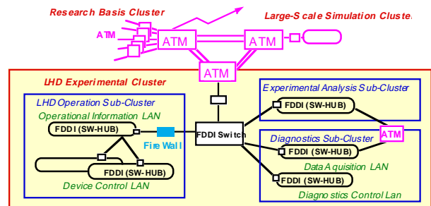
Figure 6: LHD experimental network connected to NIFS campus LAN.
