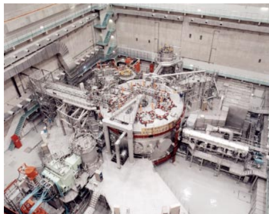
Figure1: Photograph of LHD (Large Helical Device)
