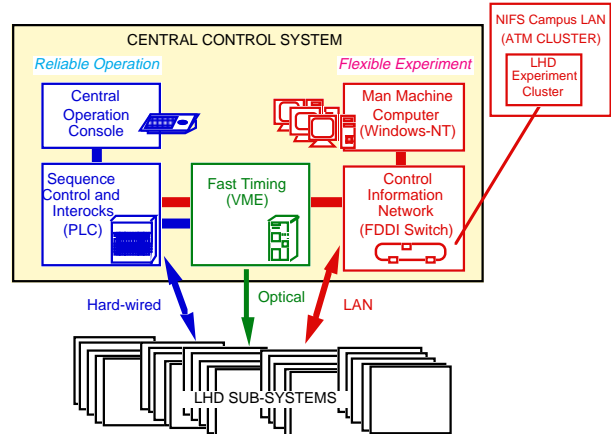
Figure 4: Outline Architecture of LHD Control.
