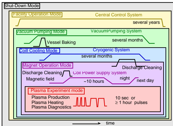
Figure 3: Six Operation Modes on LHD.
