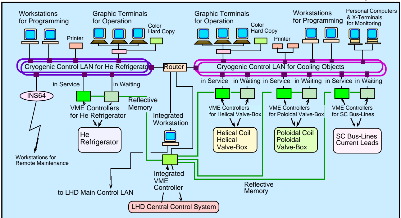
Figure 7: Cryogenic Control System
