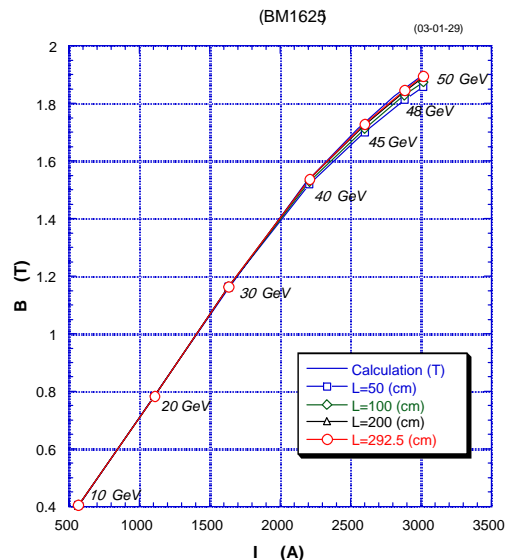
図2: 偏向電磁石のExcitation Curve (NMR)
