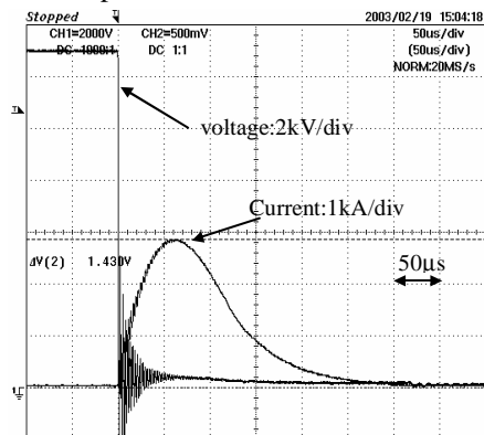
Figure7 Voltage and current wave of protection test.
