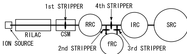
Figure 1: Schematic of RIBF.
