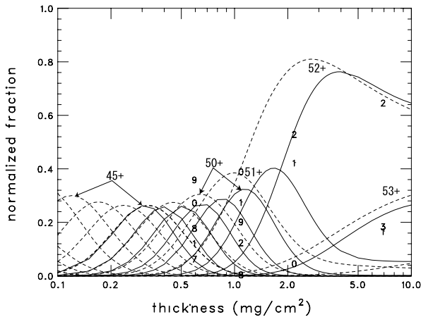
Figure 3: Charge-state fractions of ^{136}\text{Xe} at 39 MeV/nucleon stripped by carbon foils, aramid films, and a polyimide film. The definition of the axes is the same as Figure 2. Numbers without line indicate the lowest digit of measured charge-state numbers between 47+ and 53+. The charge-state fractions are normalized by the area of the Gaussian fitted to the measured charge-state distribution. Solid and dashed lines indicate the calculations by GLOBAL and ETACHA, respectively.
