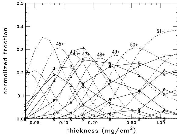
Figure 2: Charge-state fractions of ^{136}\text{Xe} at 11 MeV/nucleon stripped by carbon foils, aramid films, and a polyimide film. Horizontal and vertical axes indicate the thickness of the strippers and the charge-state fractions, respectively. Numbers joined with solid lines indicate the lowest digit of measured charge-state numbers between 42+ and 50+. The charge-state fractions are normalized by the area of the Gaussian fitted to the measured charge-state distribution. Dashed lines indicate the calculation by ETACHA.
