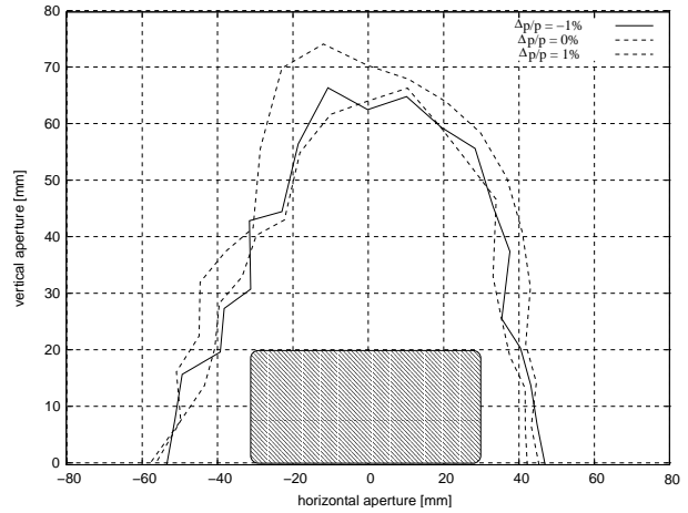
Figure 6: Results of dynamic aperture survey at 200MeV. Horizontal axis is the dynamic aperture of horizontal direction and vertical axis shows the dynamic aperture of vertical direction. Three lines shows the dynamic aperture on each of three momentum deviation ( \Delta p/p = -1\%, 0\%, 1\% ), respectively. Shadow area shows the physical aperture of synchrotron.
