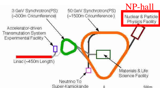
Fig. 1 Layout of the accelerator complex
