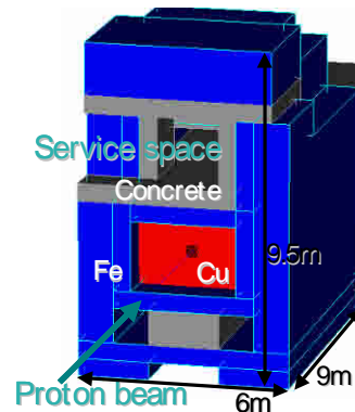
Fig. 3 Schematic view of beamdump
