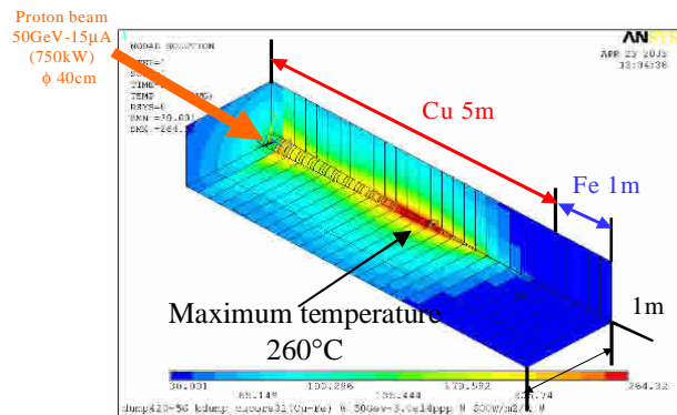
Fig. 4 Result of thermal generation
