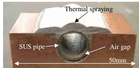
Fig. 6 Cross section of thermal spraying
