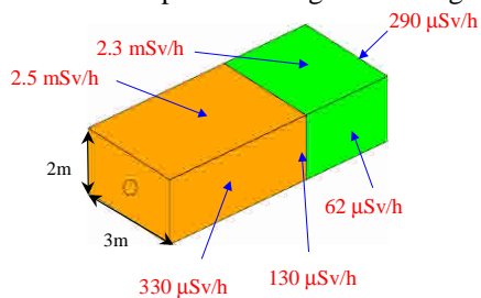
Fig. 8 calculation of residual dose rate
