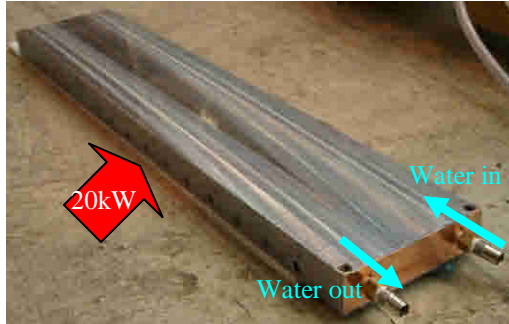
Fig.7 Mock-up for cooling test with FSW
