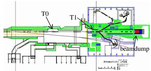
Fig. 2 Plan view of Switch Yard and NP-hall
