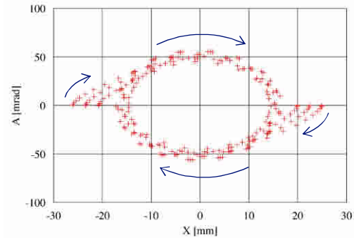
Figure 3: Phase plot of radial motion showing the capture process.
